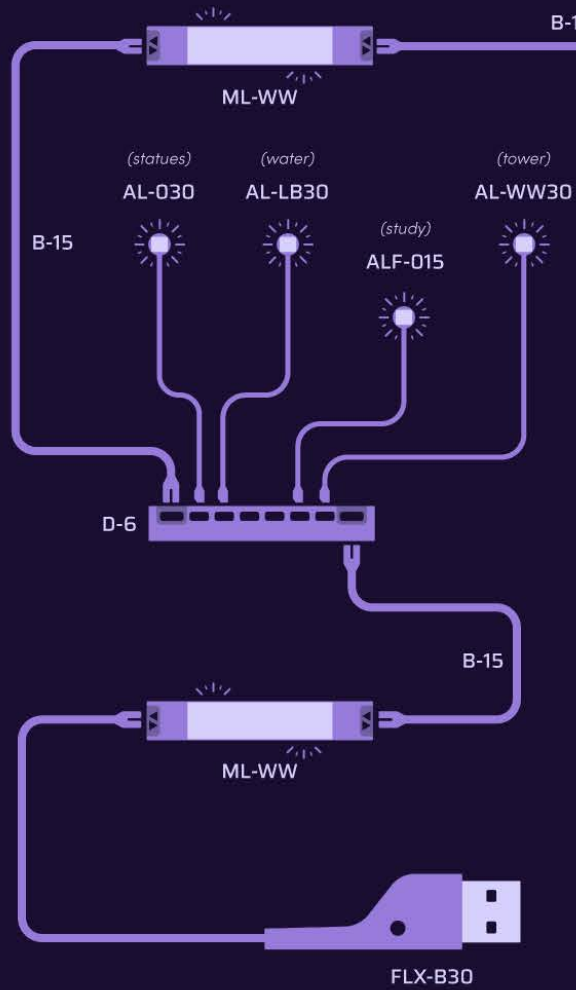
Part 1 - Tower
