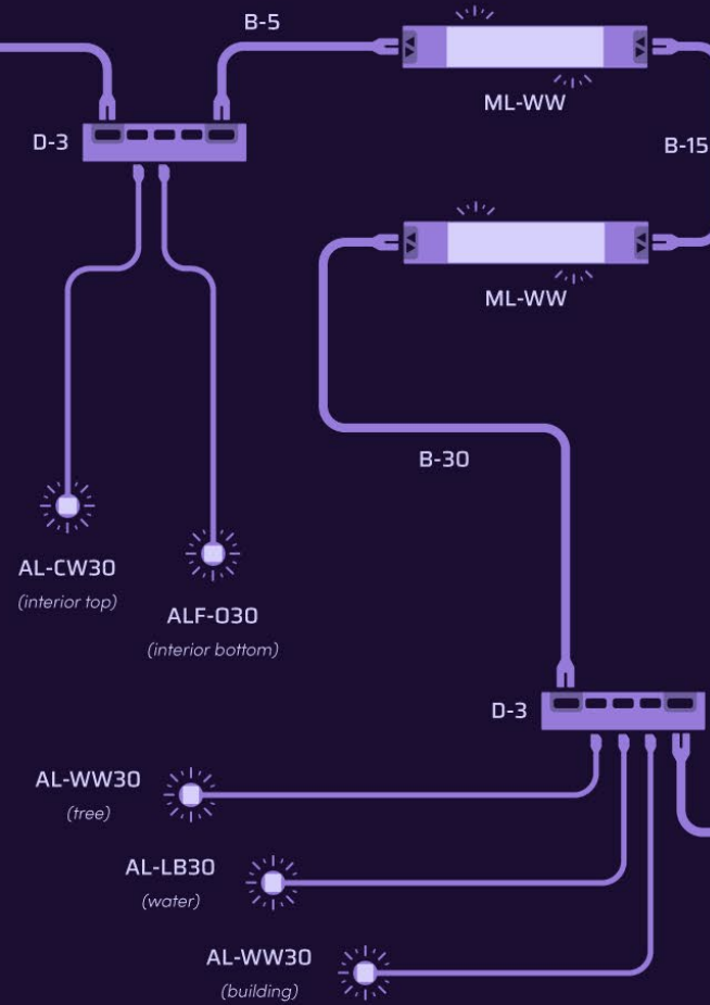
Part 2 - Hall
